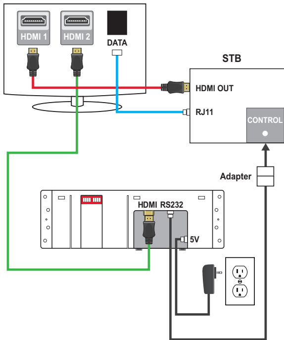
Figure 1: TV with Enseo STB cable connection diagram.
