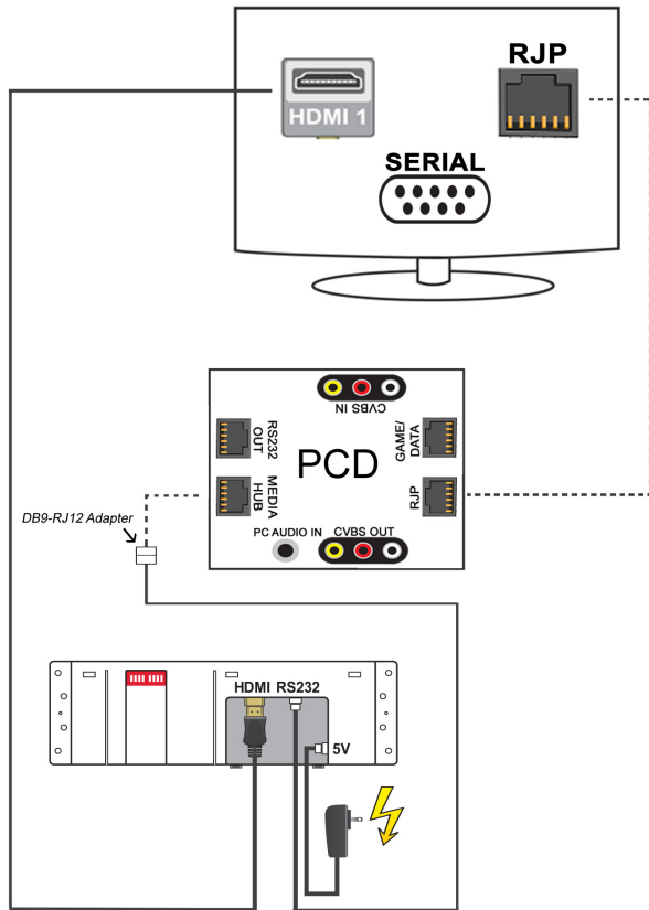
Figure 1: Cable connection diagram for installing MediaHub HD to LG RJP using the PCD.
