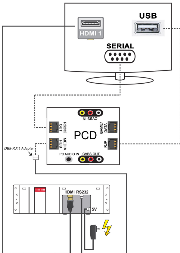
Figure 1: Cable connection diagram for installing MediaHub HD to LG Serial Control using the PCD.
