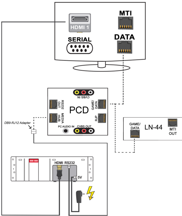
Figure 1: Cable connection diagram for installing MediaHub HD to a LodgeNet STB using the PCD.
