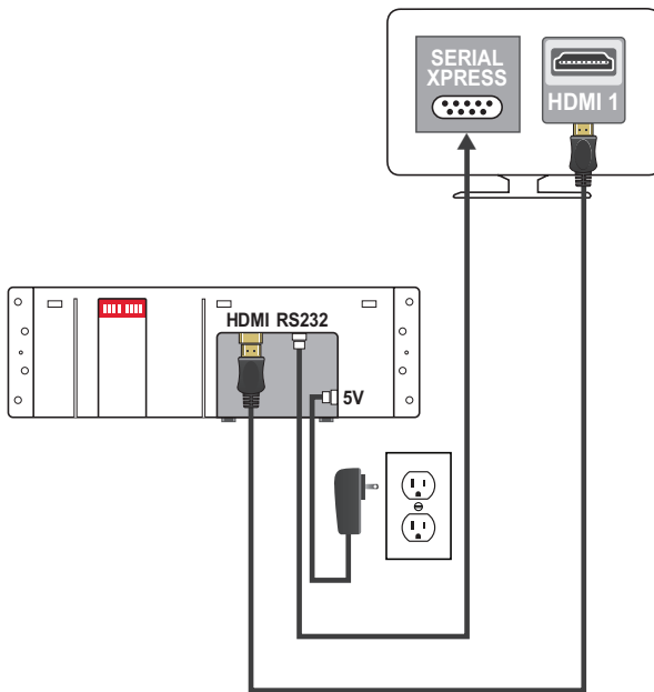
Figure 1: Philips 2009/2010 direct-to-TV cable connection diagram.
